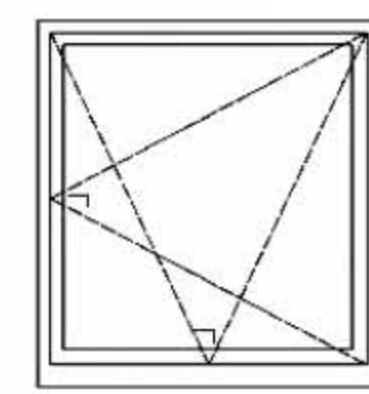
Tilt In Turn Out
